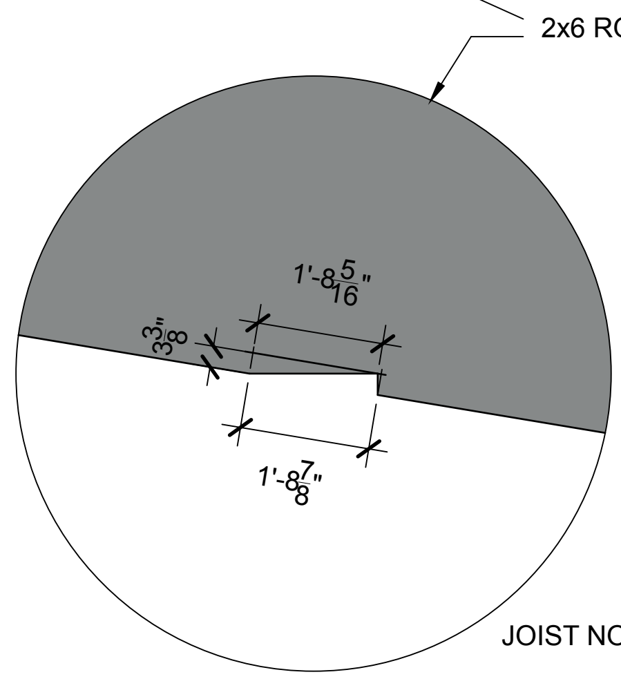
JOIST END ANGLE DETAIL
